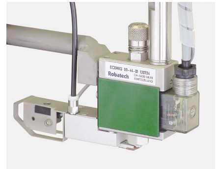
ECXMKs: 16 mm bracket and nozzle cover slider
