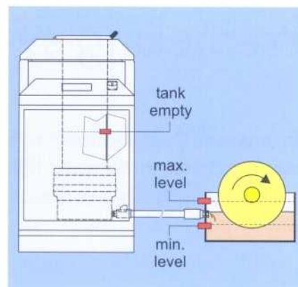
Principle diagram with level sensors
